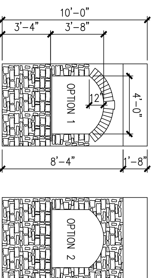
ELEVATION @ BUTLER PANTRY SCALE: 1/4" = 1'-0"
