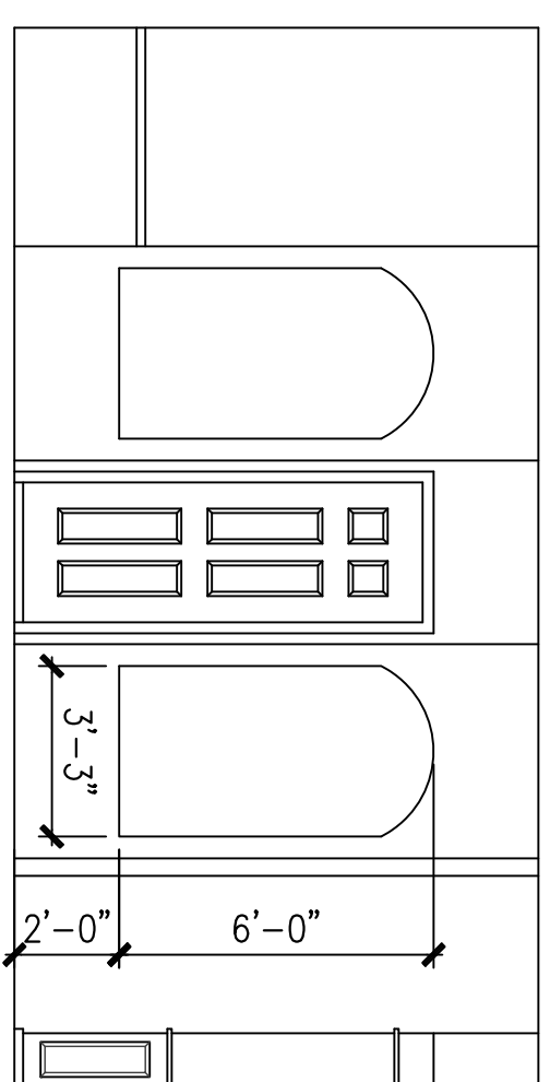
ELEVATION @ HALL SCALE: 1/4" = 1'-0"
