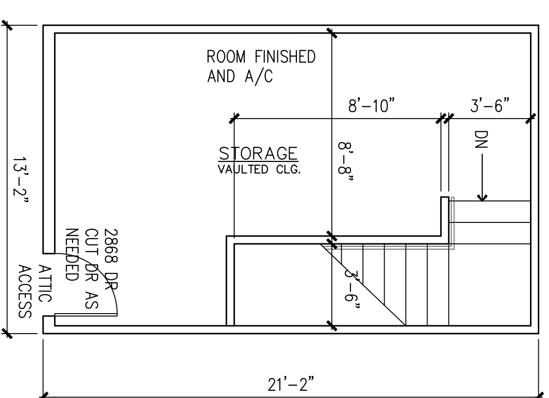
2nd STORAGE PLAN SCALE: 1/4" = 1'-0"
