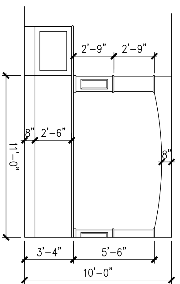
ELEVATION @ LIVING RM SCALE: 1/4" = 1'-0"
