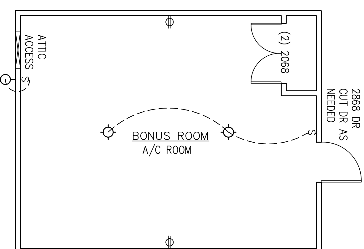
BONUS ROOM PLAN SCALE: 1/4" = 1'-0"
