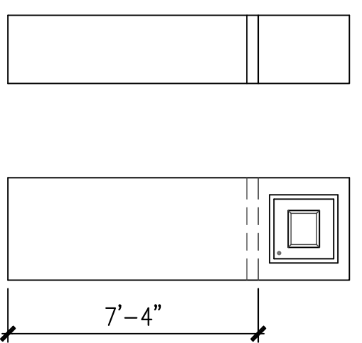
ELEVATION @ DEN CLOSET SCALE: 1/4" = 1'-0"
