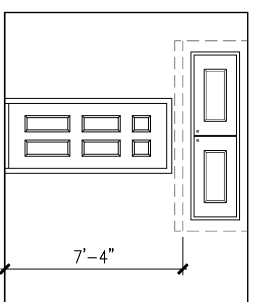
ELEVATION @ BEDROOM SCALE: 1/4" = 1'-0"
